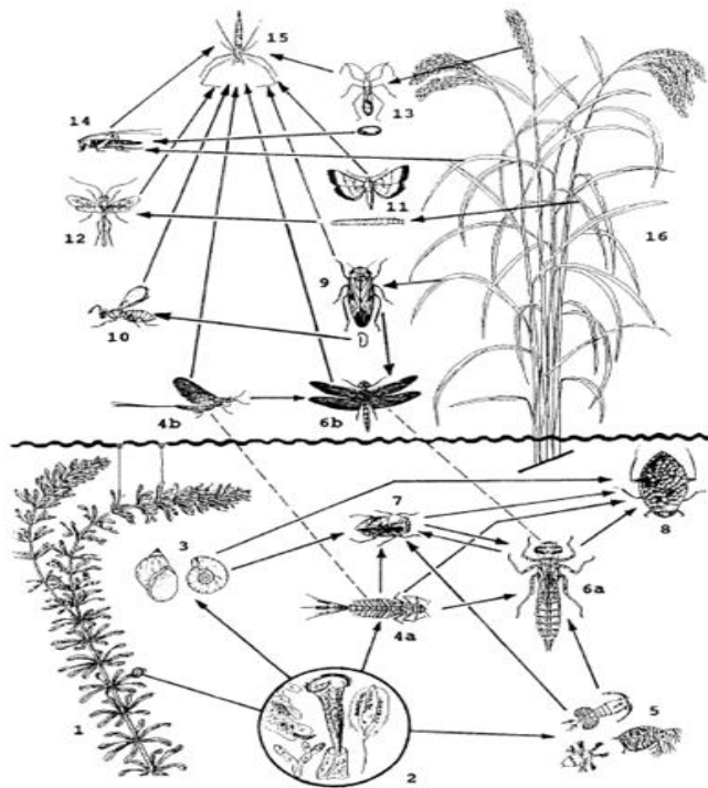
Figure 2. Food web of an Ifugao agro-ecosystem (Setelle and Martin, 1998)
